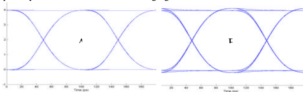
Figure 3. Effect of overshoot on extinction ratio
