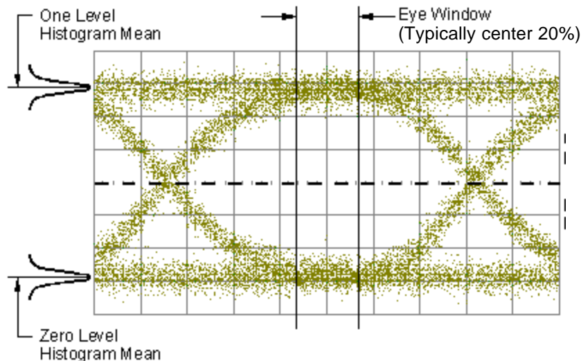
Figure 1. Definition of extinction ratio
